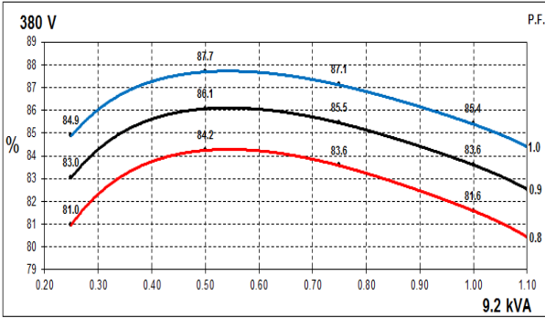
50Hz Curves
