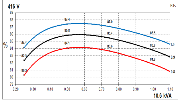
60Hz Curves
